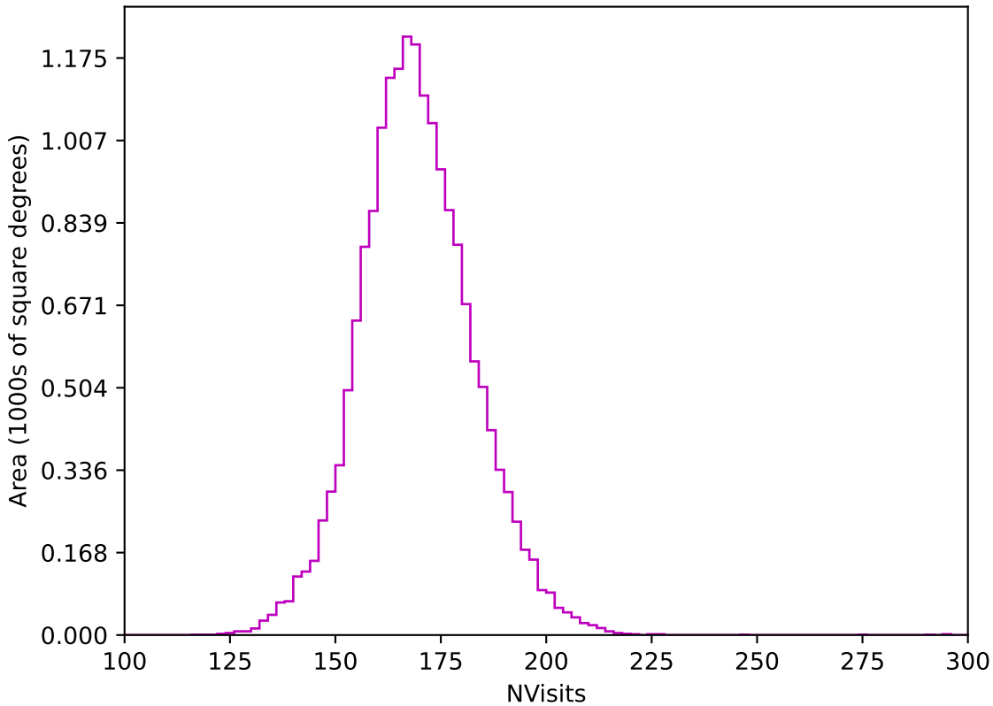
too_elab_heavy_r32_d3_ugrizy_v3.4_10yrs WFD z band: NVisits
