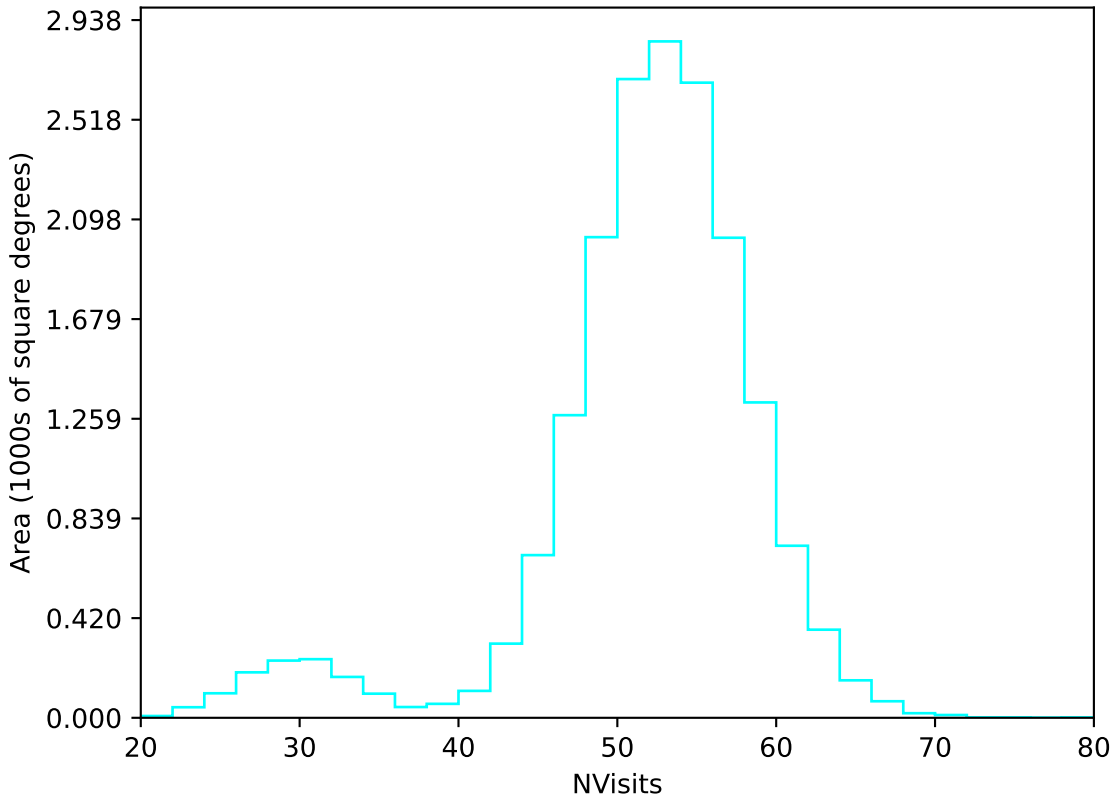
too_elab_heavy_r32_d3_ugrizy_v3.4_10yrs WFD u band: NVisits
