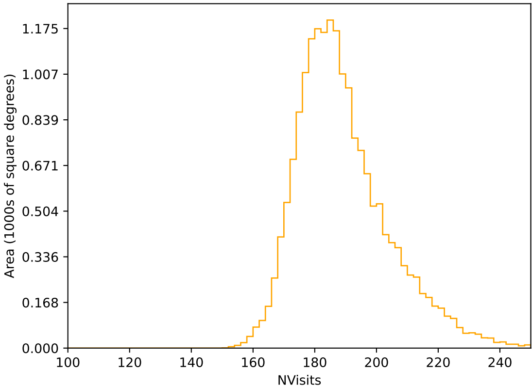
too_elab_heavy_r32_d3_ugrizy_v3.4_10yrs WFD r band: NVisits
