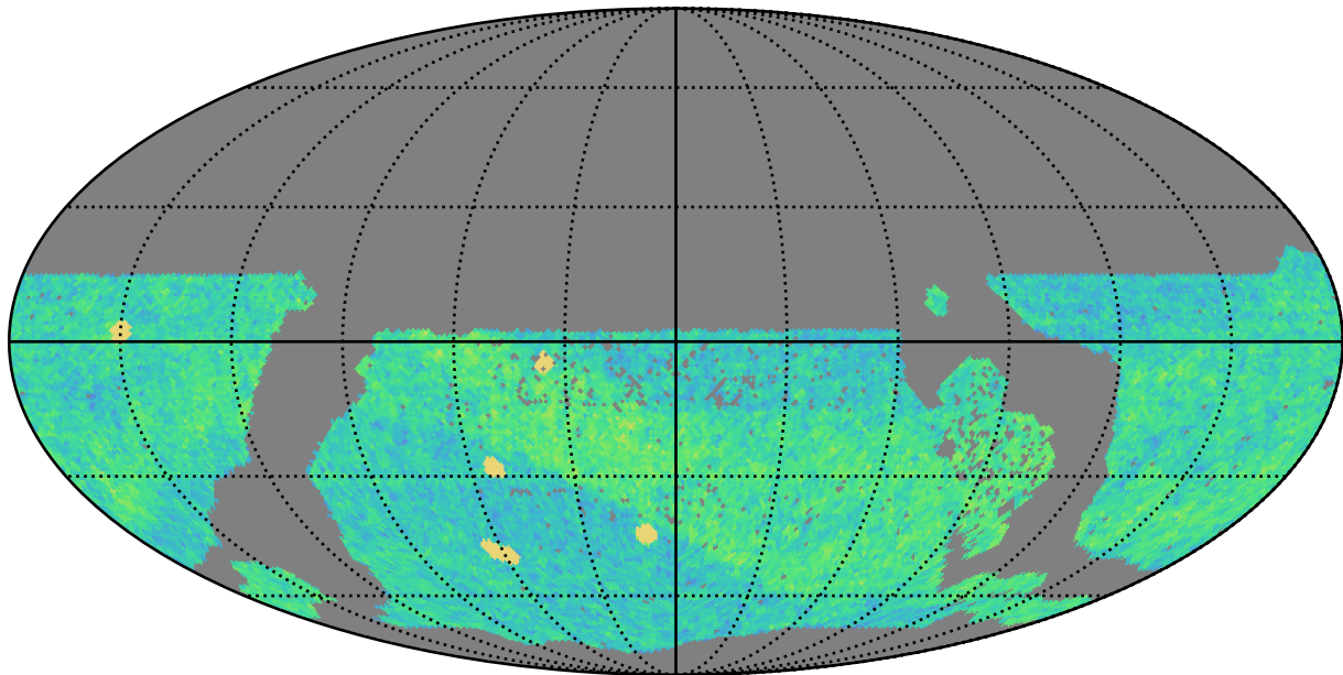
too_elab_heavy_r32_d3_ugrizy_v3.4_10yrs WFD i band: NVisits
