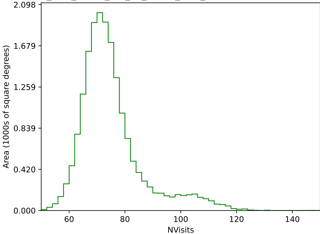
too_elab_heavy_r32_d3_ugrizy_v3.4_10yrs WFD g band: NVisits
