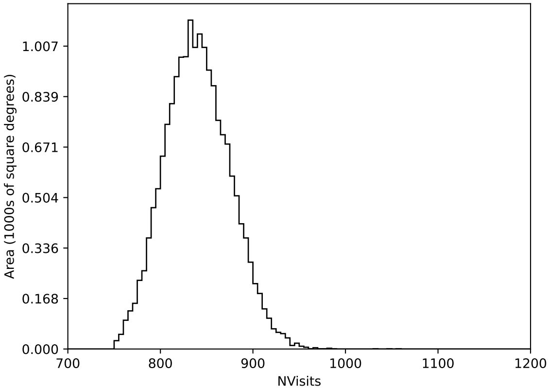
too_elab_heavy_r32_d3_ugrizy_v3.4_10yrs WFD all bands: NVisits
