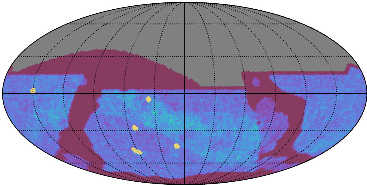
too_elab_heavy_r32_d3_ugrizy_v3.4_10yrs All sky z band: NVisits
