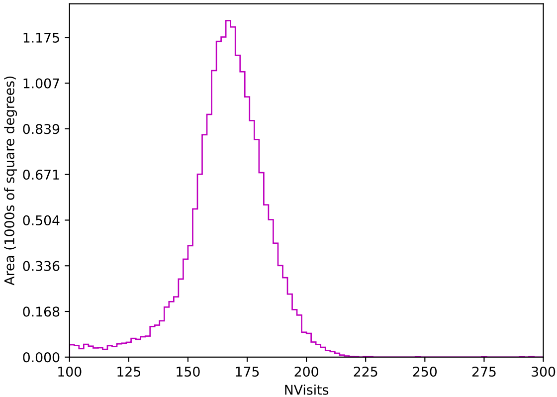
too_elab_heavy_r32_d3_ugrizy_v3.4_10yrs All sky z band: NVisits
