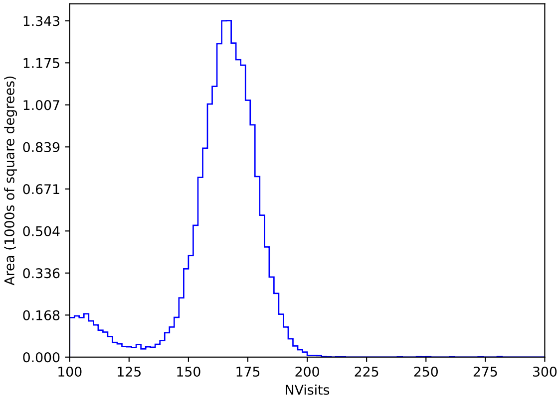
too_elab_heavy_r32_d3_ugrizy_v3.4_10yrs All sky y band: NVisits
