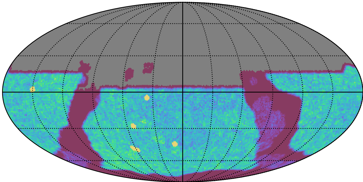
too_elab_heavy_r32_d3_ugrizy_v3.4_10yrs All sky u band: NVisits
