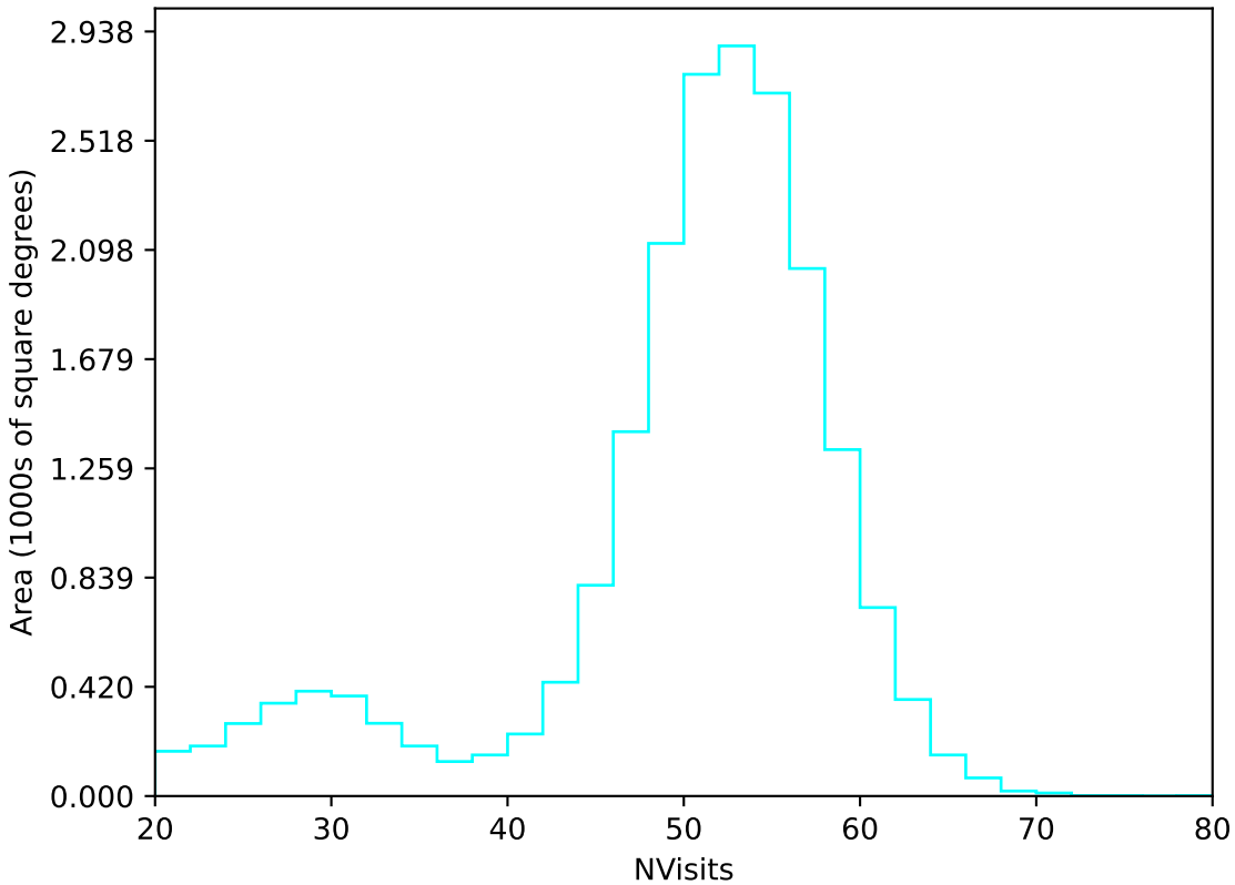
too_elab_heavy_r32_d3_ugrizy_v3.4_10yrs All sky u band: NVisits
