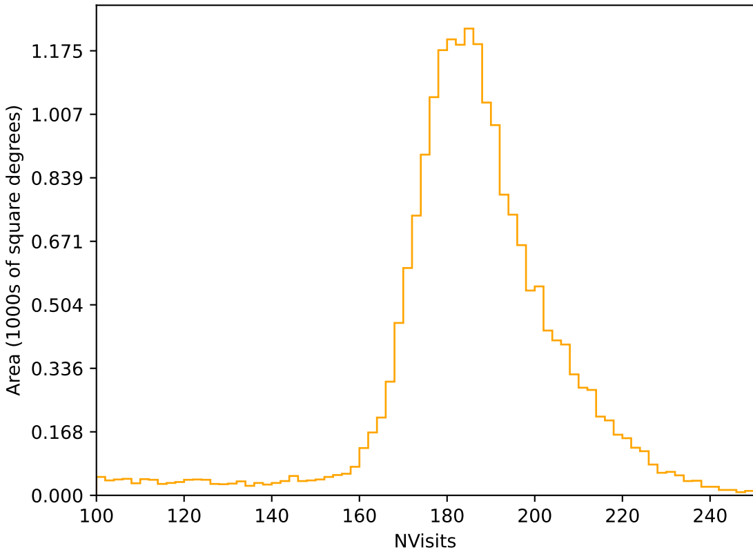
too_elab_heavy_r32_d3_ugrizy_v3.4_10yrs All sky r band: NVisits
