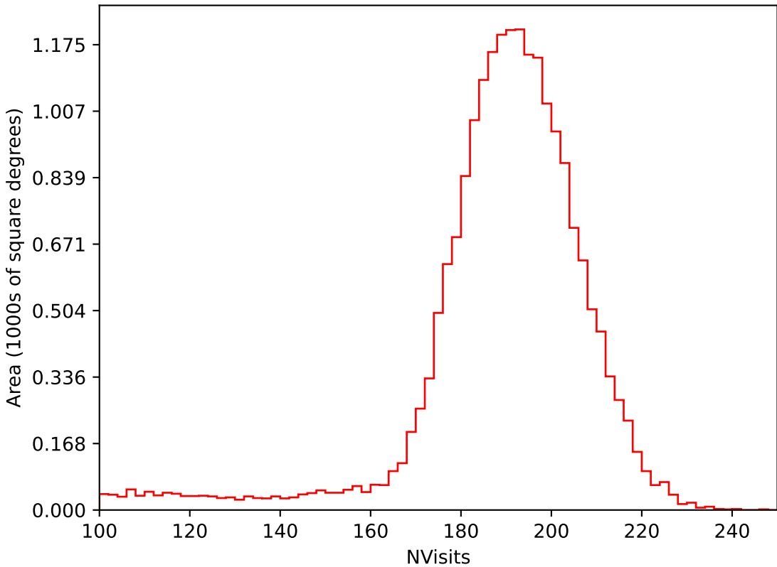
too_elab_heavy_r32_d3_ugrizy_v3.4_10yrs All sky i band: NVisits
