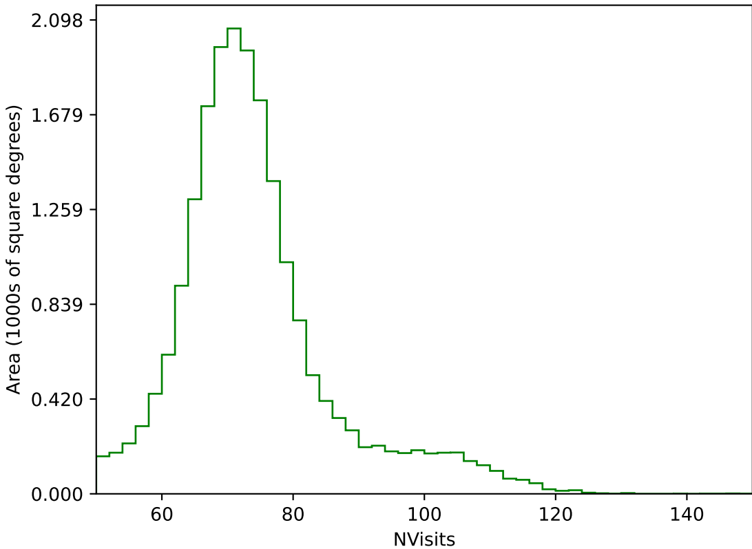
too_elab_heavy_r32_d3_ugrizy_v3.4_10yrs All sky g band: NVisits
