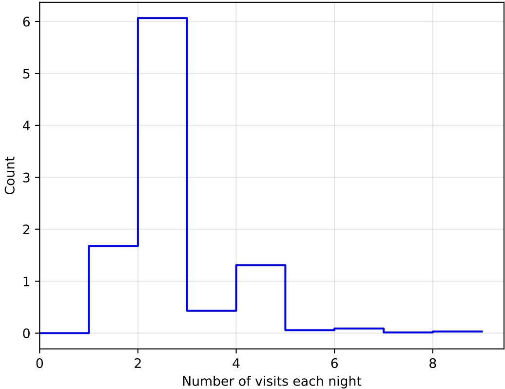
too_elab_heavy_r32_d3_ugrizy_v3.4_10yrs All sky: NVisitsPerNight 1e6
