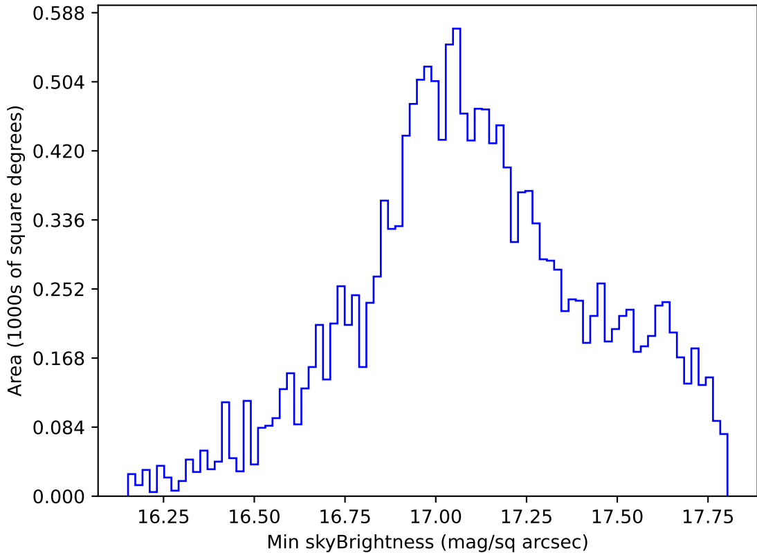
too_elab_heavy_r32_d3_ugrizy_v3.4_10yrs WFD y band: Min skyBrightness
