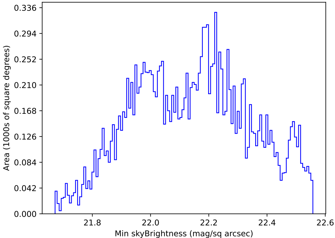
too_elab_heavy_r32_d3_ugrizy_v3.4_10yrs WFD u band: Min skyBrightness
