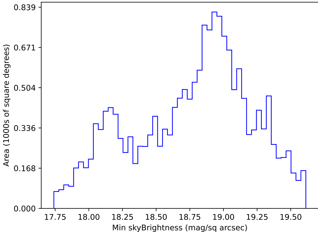
too_elab_heavy_r32_d3_ugrizy_v3.4_10yrs WFD r band: Min skyBrightness
