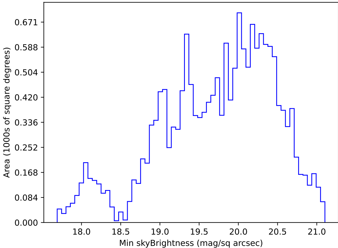
too_elab_heavy_r32_d3_ugrizy_v3.4_10yrs WFD g band: Min skyBrightness
