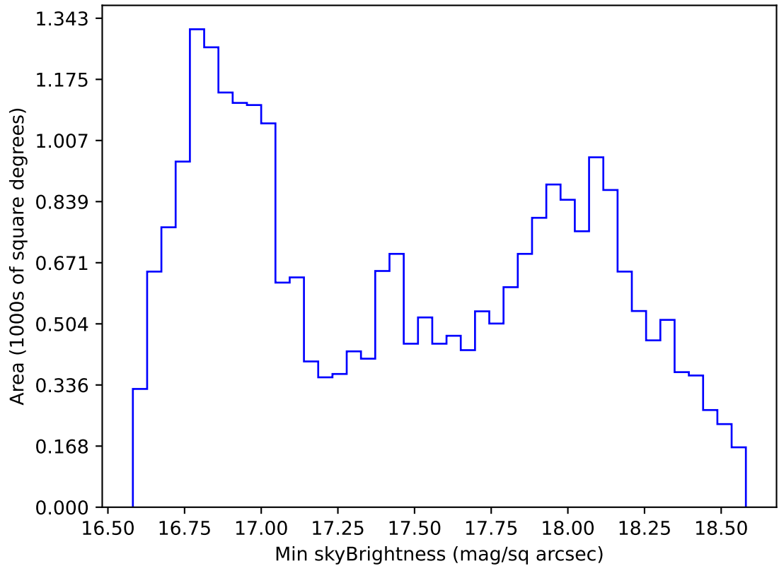
too_elab_heavy_r32_d3_ugrizy_v3.4_10yrs All sky z band: Min skyBrightness
