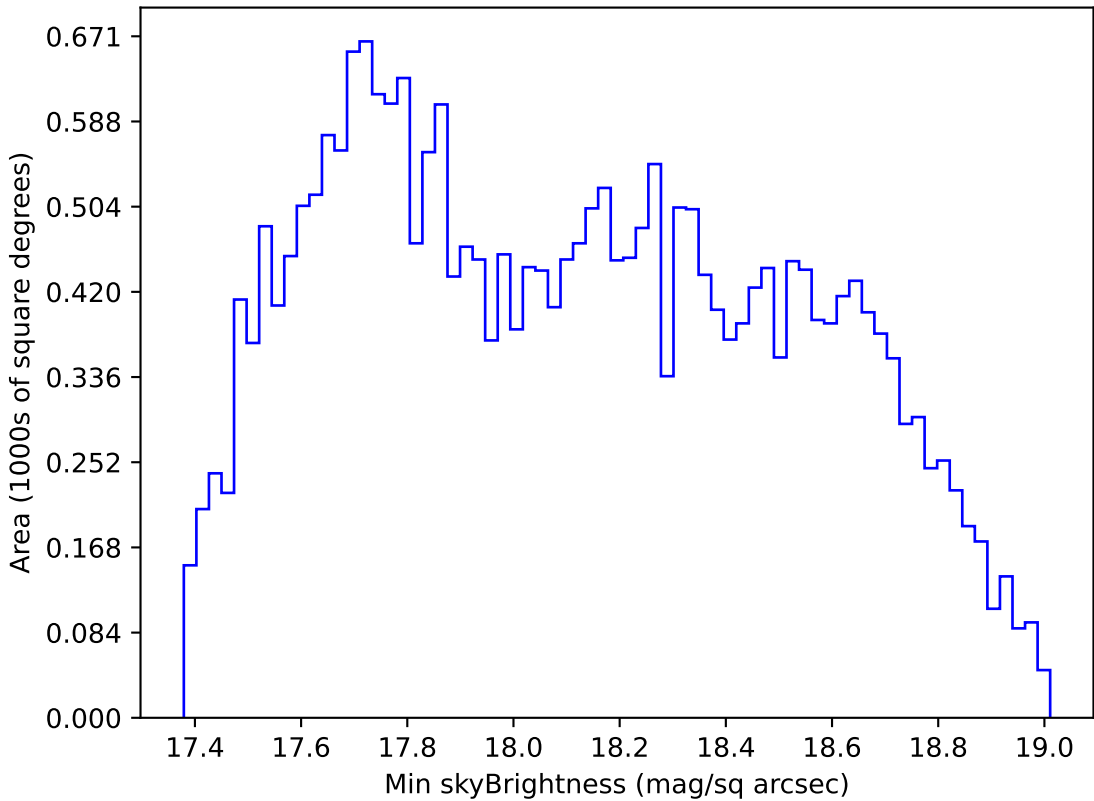
too_elab_heavy_r32_d3_uigrizy_v3.4_10yrs All sky i band: Min skyBrightness
