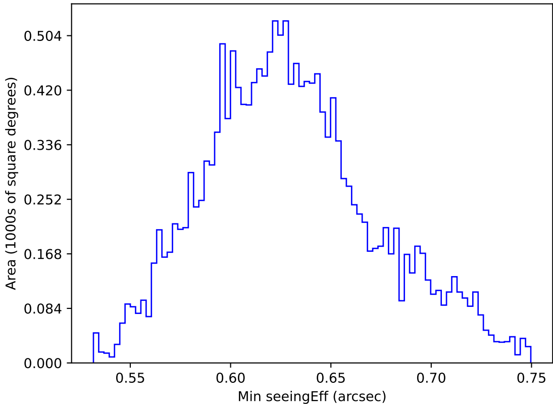
too_elab_heavy_r32_d3_ugrizy_v3.4_10yrs WFD y band: Min seeingEff
