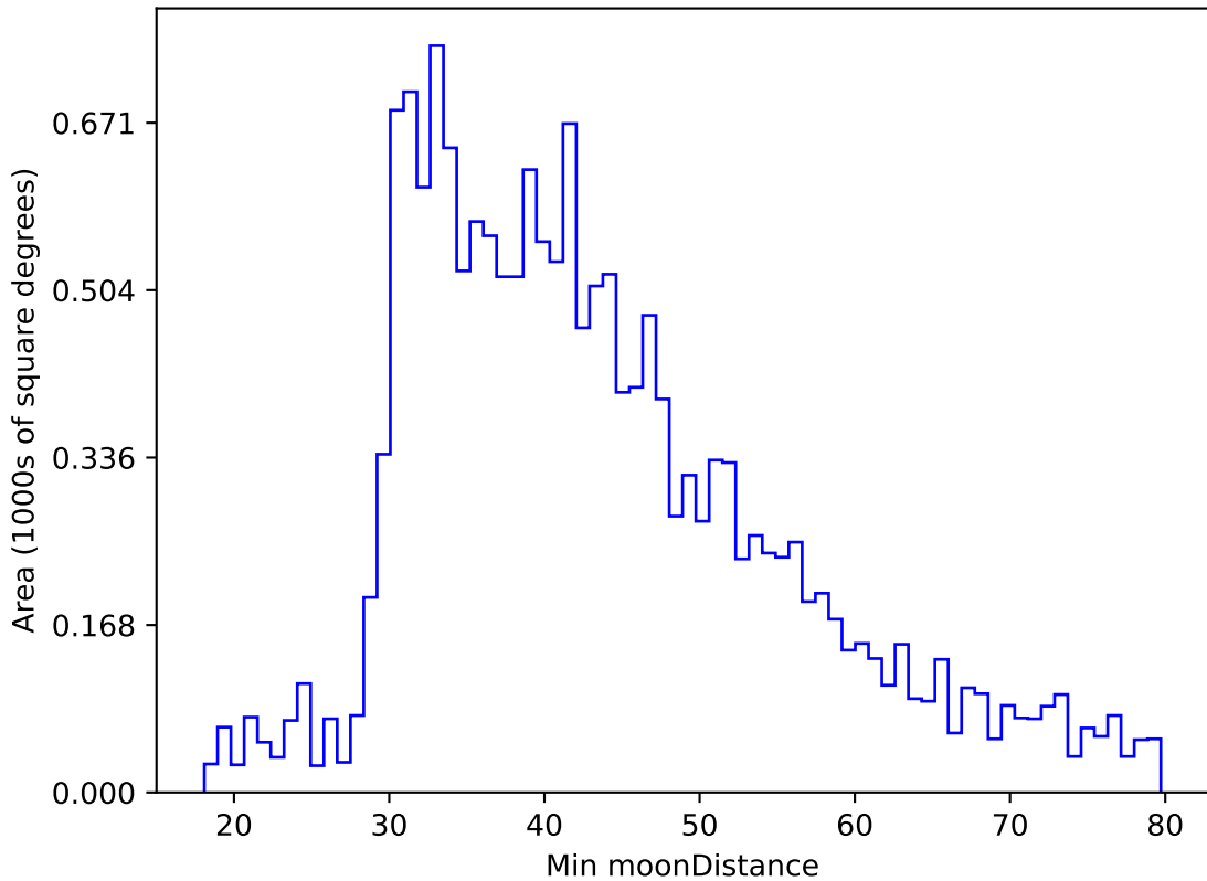
too_elab_heavy_r32_d3_ugrizy_v3.4_10yrs WFD g band: Min moonDistance
