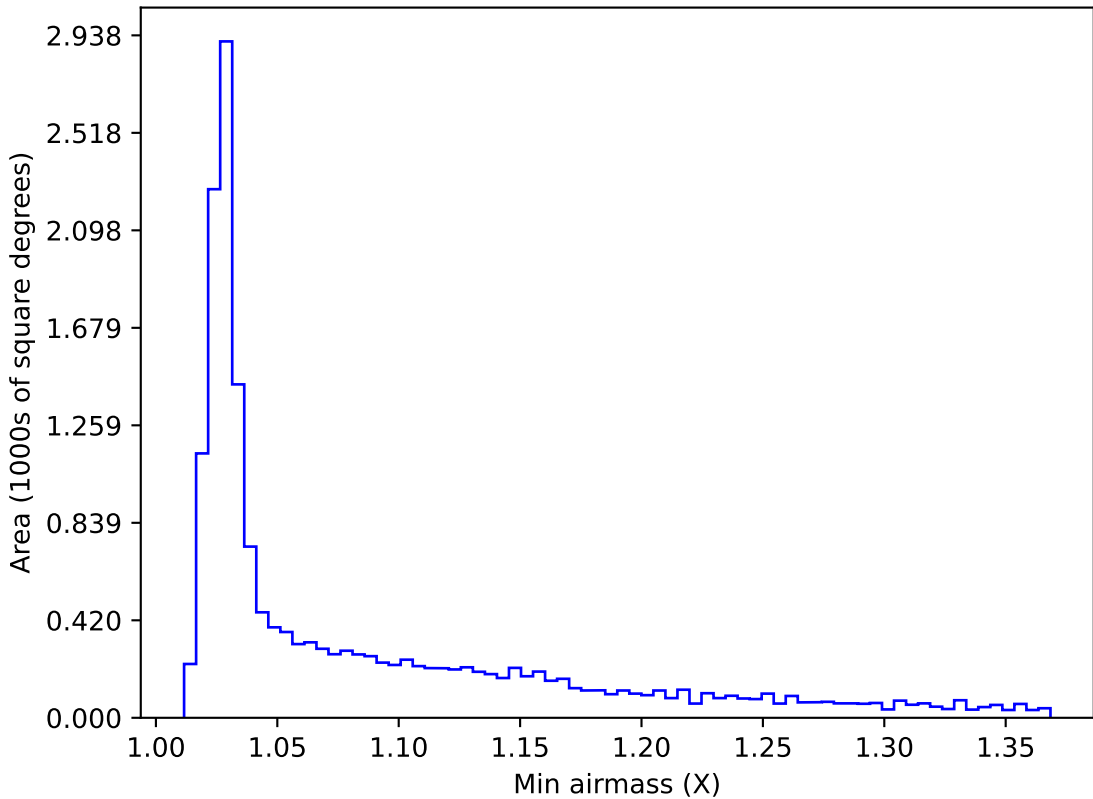
too_elab_heavy_r32_d3_ugrizy_v3.4_10yrs WFD r band: Min airmass
