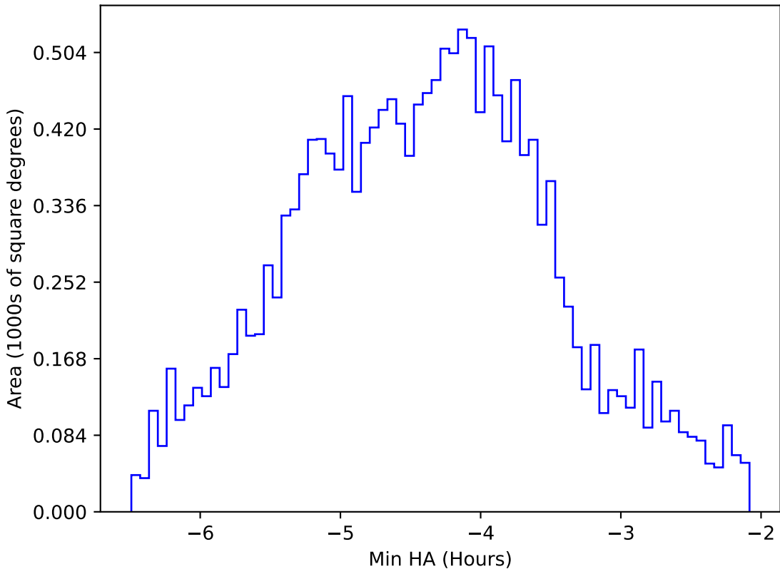
too_elab_heavy_r32_d3_ugrizy_v3.4_10yrs WFD z band: Min HA
