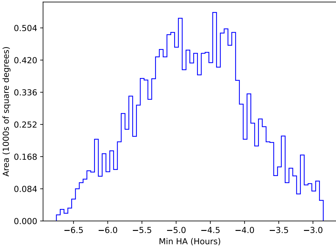
too_elab_heavy_r32_d3_ugrizy_v3.4_10yrs WFD all bands: Min HA
