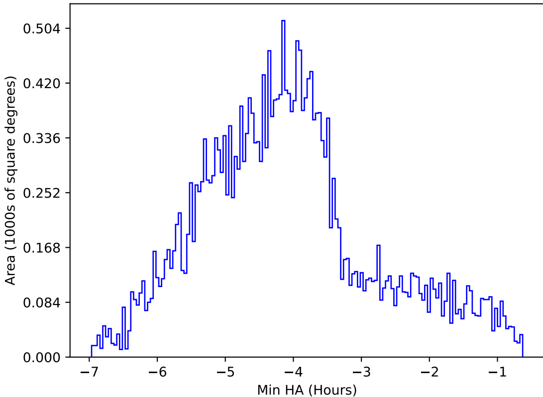
too_elab_heavy_r32_d3_ugrizy_v3.4_10yrs All sky z band: Min HA
