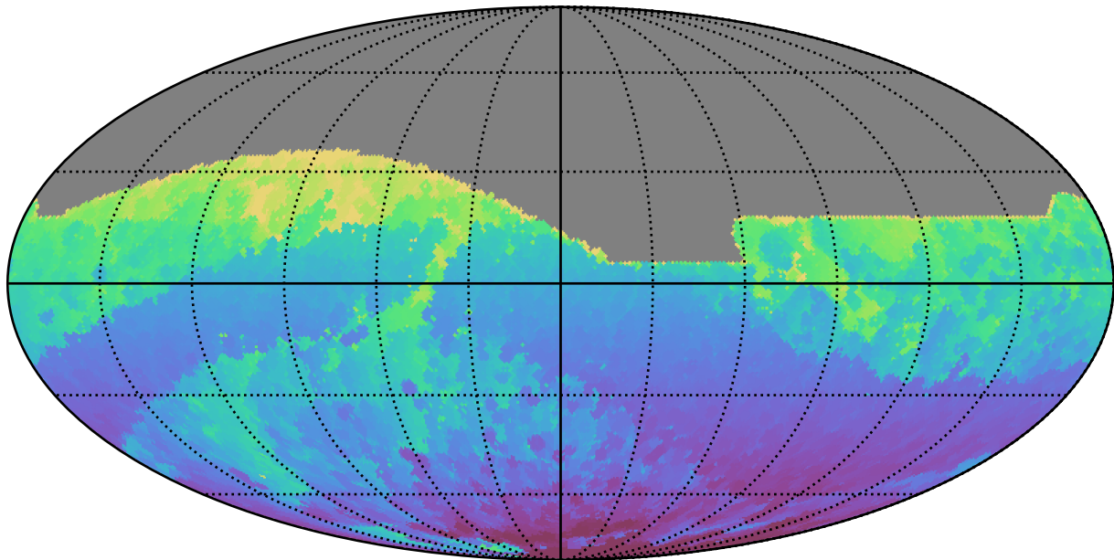
too_elab_heavy_r32_d3_ugrizy_v3.4_10yrs All sky r band: Min HA
