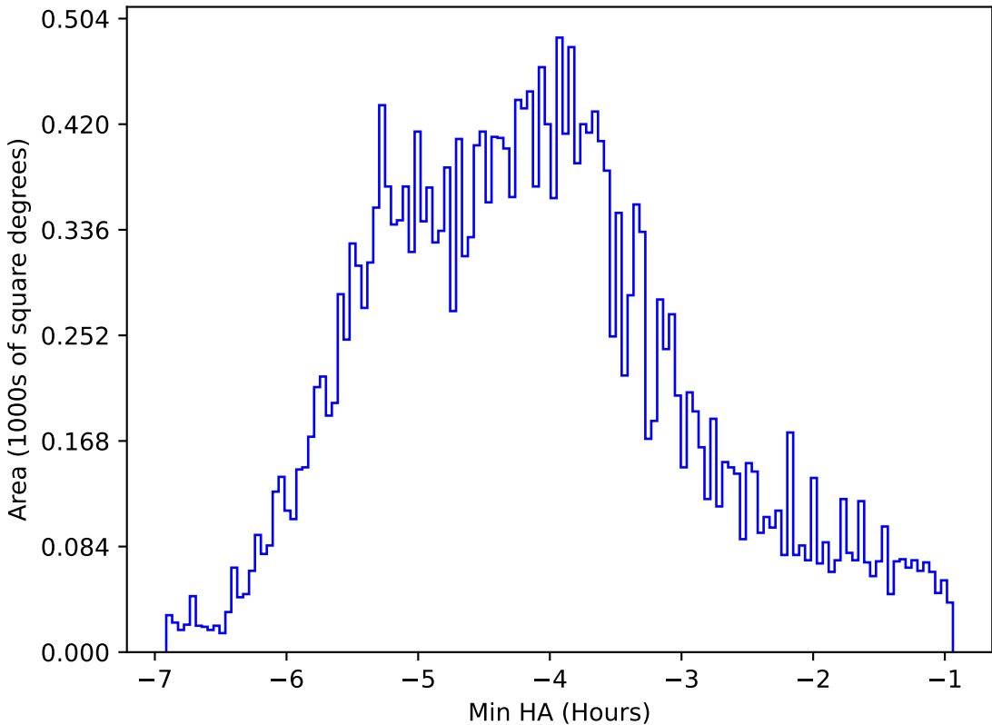
too_elab_heavy_r32_d3_ugrizy_v3.4_10yrs All sky r band: Min HA
