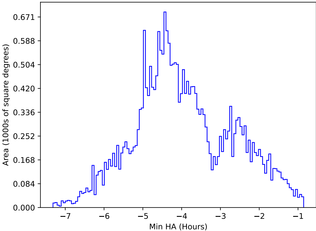
too_elab_heavy_r32_d3_ugrizy_v3.4_10yrs All sky g band: Min HA
