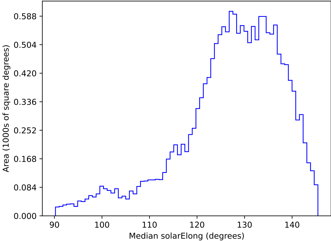
too_elab_heavy_r32_d3_ugrizy_v3.4_10yrs WFD z band: Median solarElong
