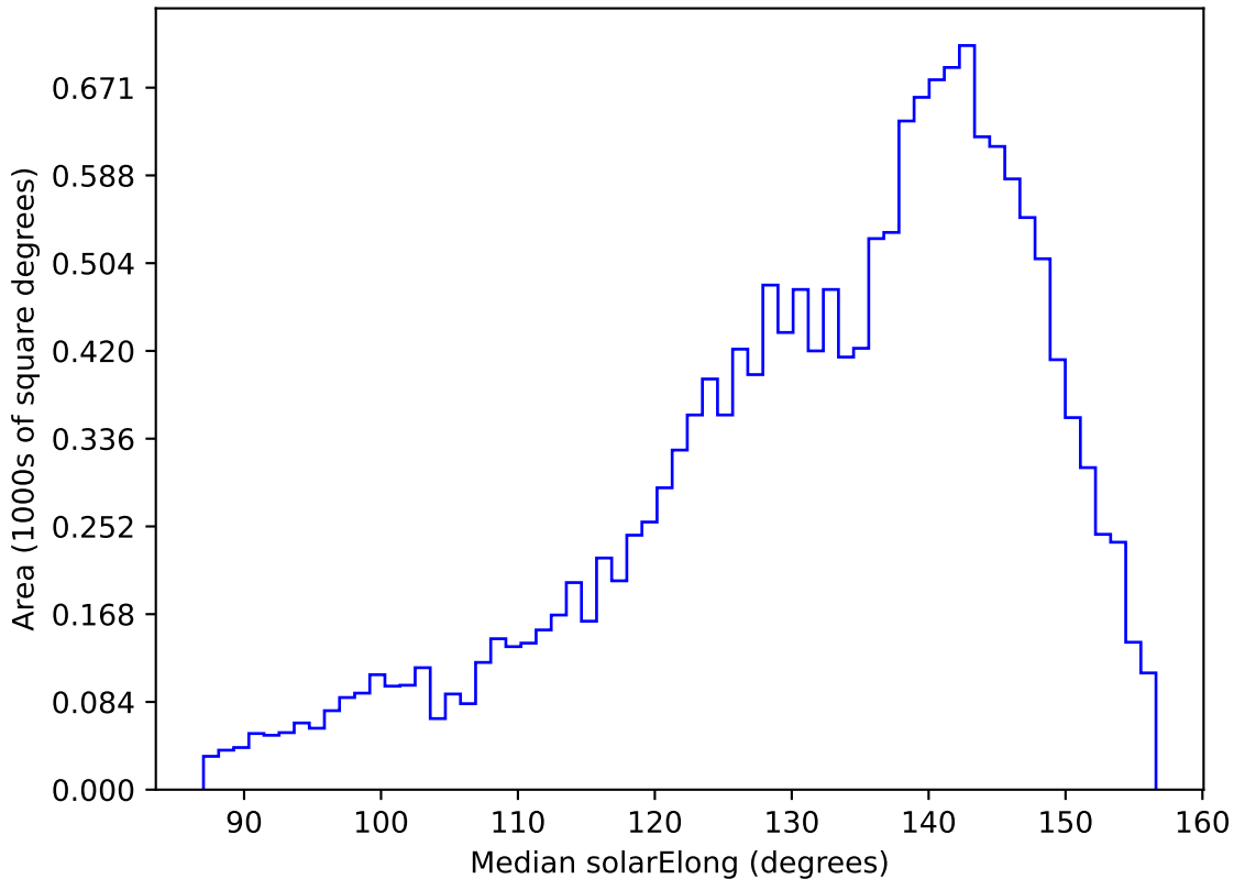
too_elab_heavy_r32_d3_ugrizy_v3.4_10yrs WFD u band: Median solarElong
