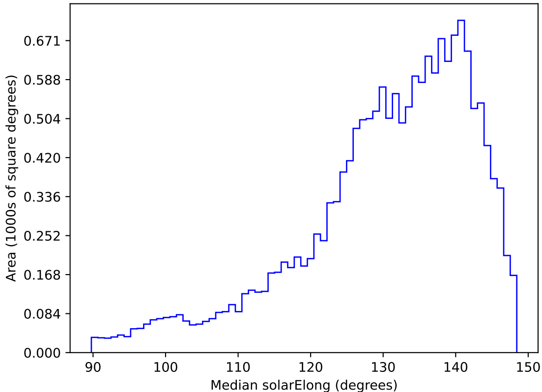
too_elab_heavy_r32_d3_ugrizy_v3.4_10yrs WFD r band: Median solarElong
