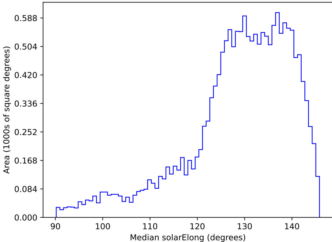
too_elab_heavy_r32_d3_ugrizy_v3.4_10yrs WFD i band: Median solarElong
