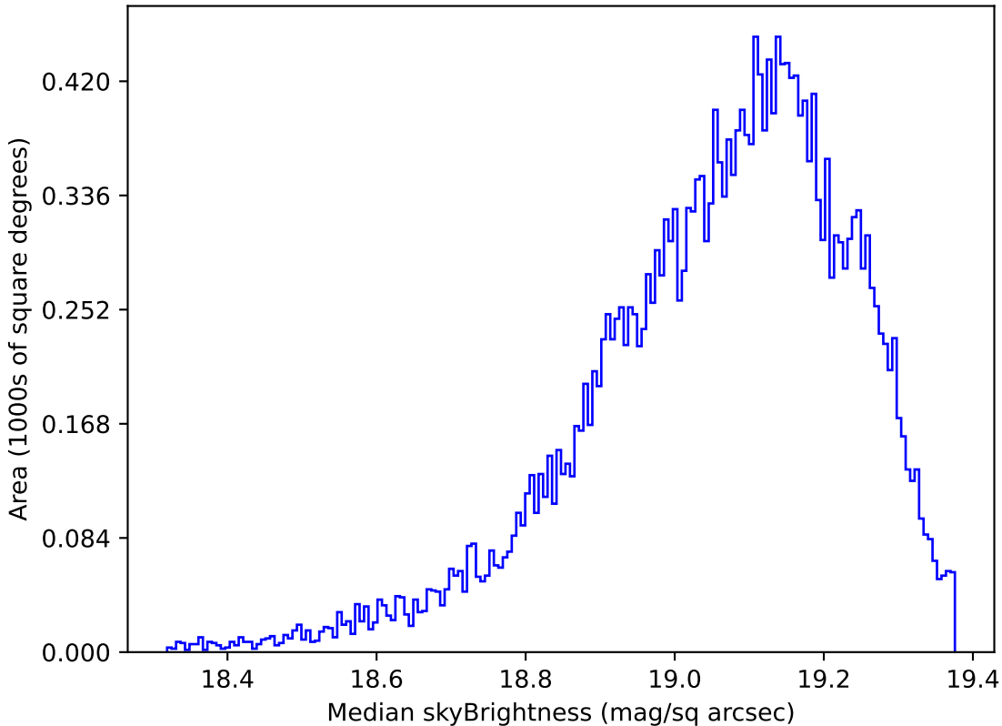
too_elab_heavy_r32_d3_ugrizy_v3.4_10yrs Yr 1 z band: Median skyBrightness
