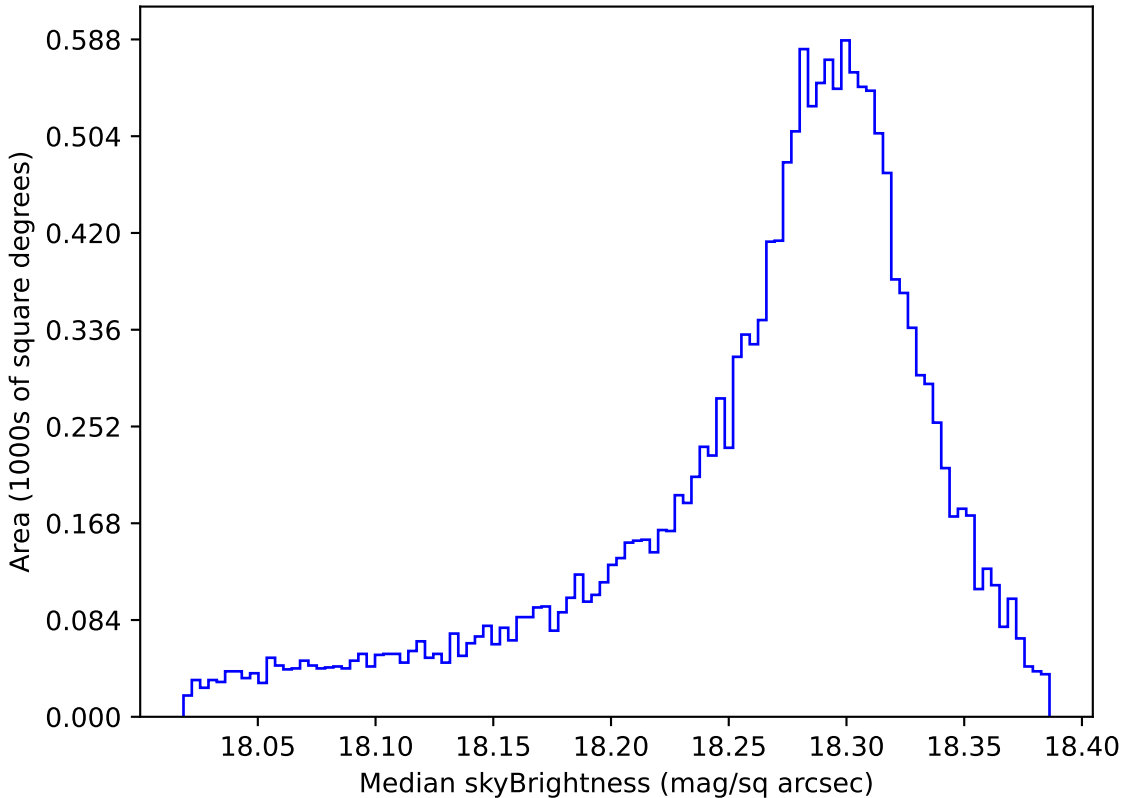
too_elab_heavy_r32_d3_ugrizy_v3.4_10yrs WFD y band: Median skyBrightness
