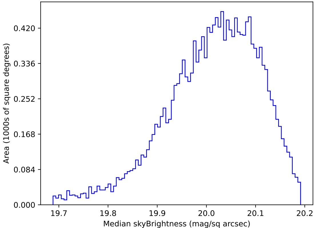
too_elab_heavy_r32_d3_ugrizy_v3.4_10yrs WFD i band: Median skyBrightness
