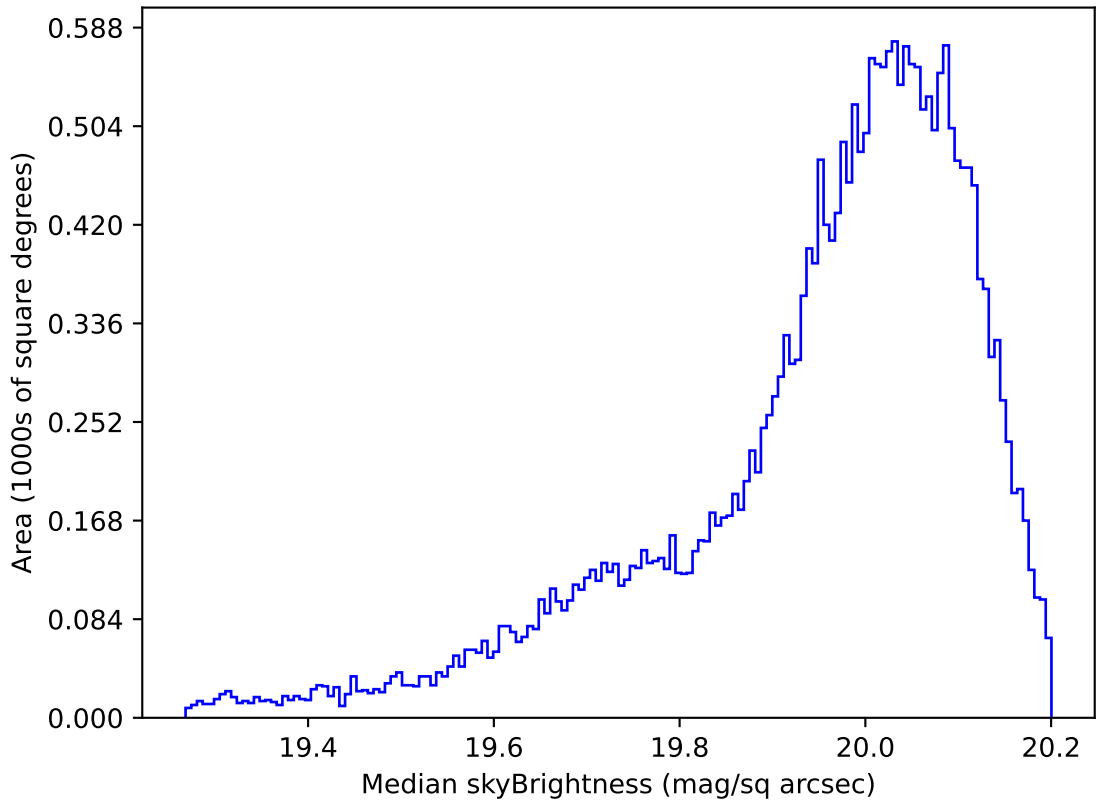
too_elab_heavy_r32_d3_ugrizy_v3.4_10yrs All sky i band: Median skyBrightness
