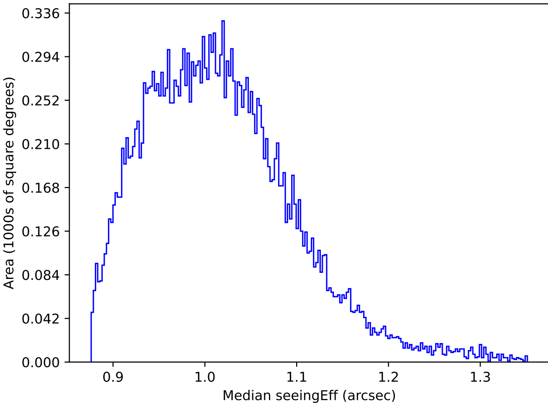
too_elab_heavy_r32_d3_ugrizy_v3.4_10yrs All sky y band: Median seeingEff
