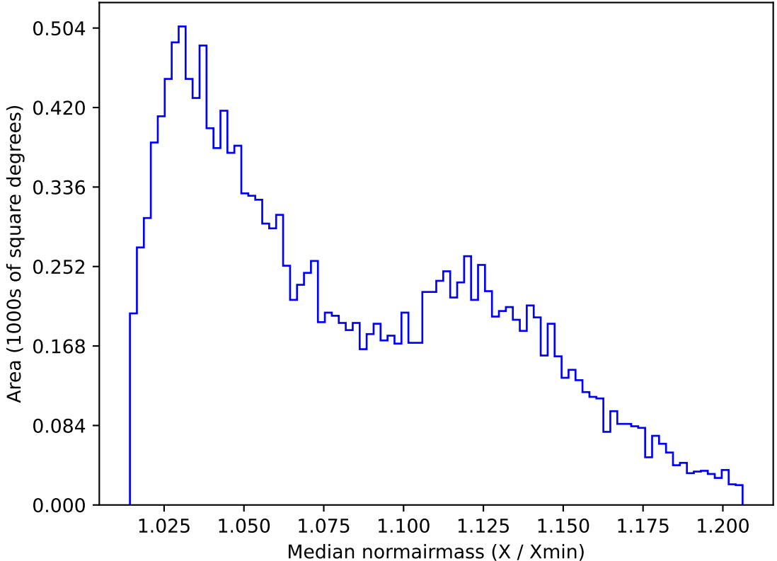
too_elab_heavy_r32_d3_ugrizy_v3.4_10yrs WFD u band: Median normairmass
