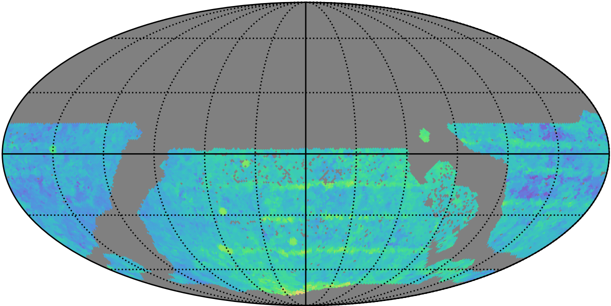
too_elab_heavy_r32_d3_ugrizy_v3.4_10yrs WFD z band: Median Season Length
