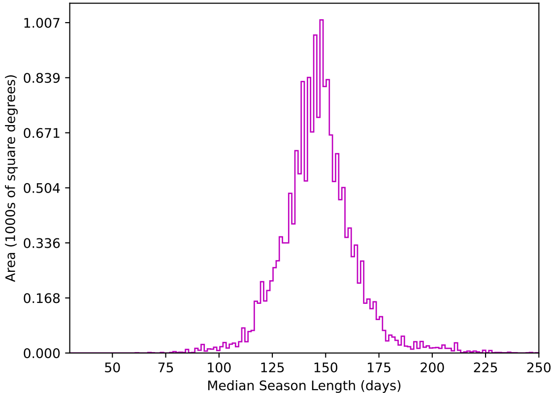
too_elab_heavy_r32_d3_ugrizy_v3.4_10yrs WFD z band: Median Season Length
