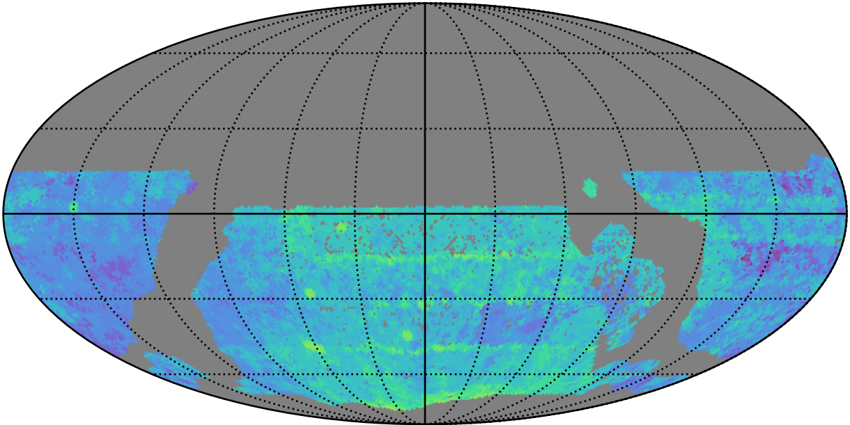
too_elab_heavy_r32_d3_ugrizy_v3.4_10yrs WFD y band: Median Season Length
