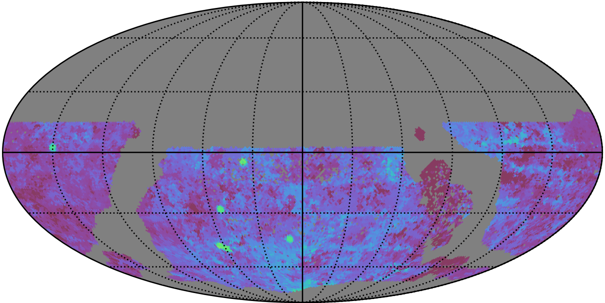
too_elab_heavy_r32_d3_ugrizy_v3.4_10yrs WFD u band: Median Season Length
