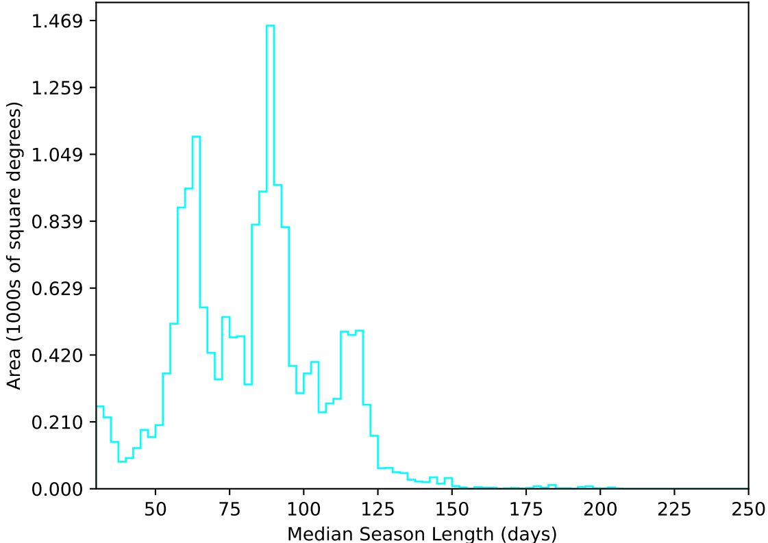
too_elab_heavy_r32_d3_ugrizy_v3.4_10yrs WFD u band: Median Season Length
