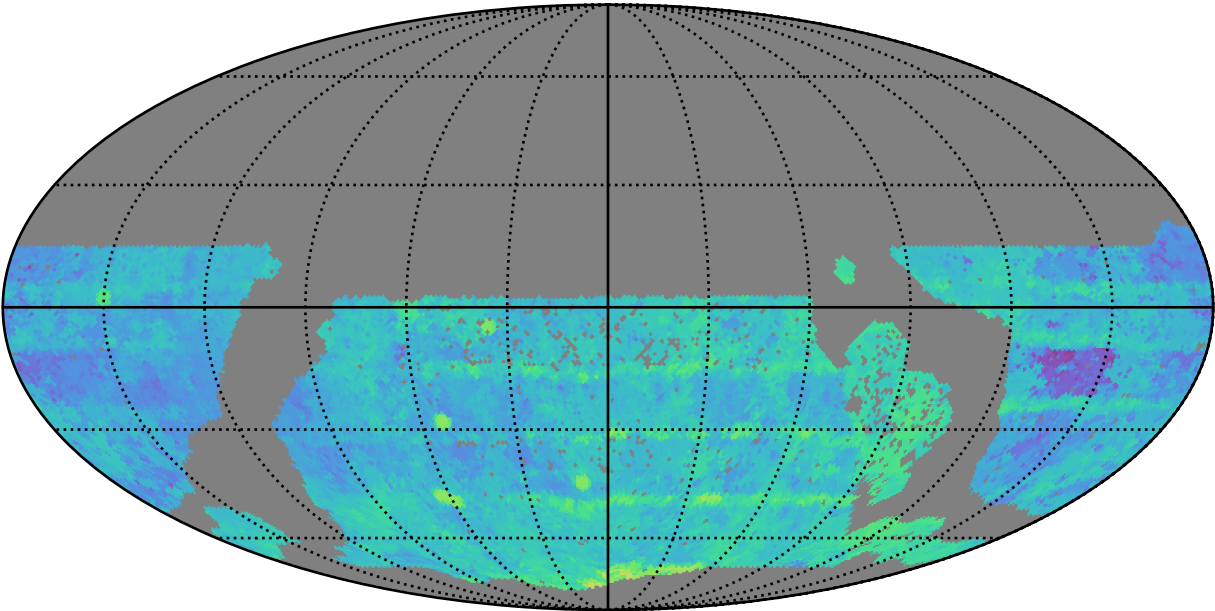
too_elab_heavy_r32_d3_ugrizy_v3.4_10yrs WFD r band: Median Season Length
