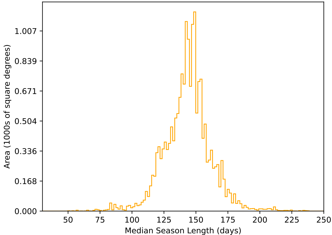
too_elab_heavy_r32_d3_ugrizy_v3.4_10yrs WFD r band: Median Season Length
