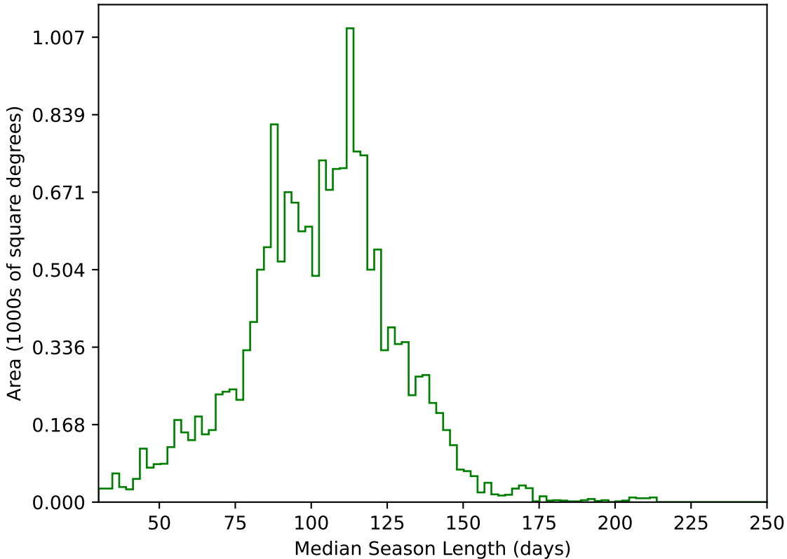
too_elab_heavy_r32_d3_ugrizy_v3.4_10yrs WFD g band: Median Season Length
