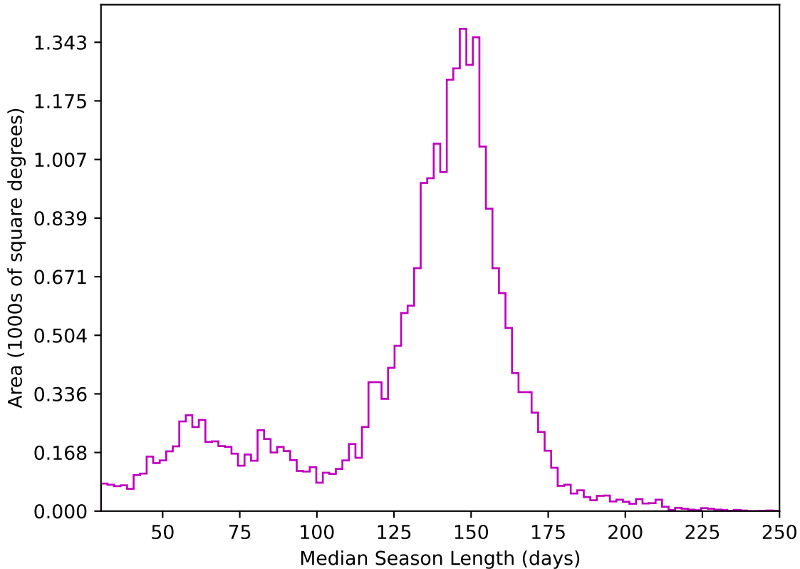
too_elab_heavy_r32_d3_ugrizy_v3.4_10yrs All sky z band: Median Season Length
