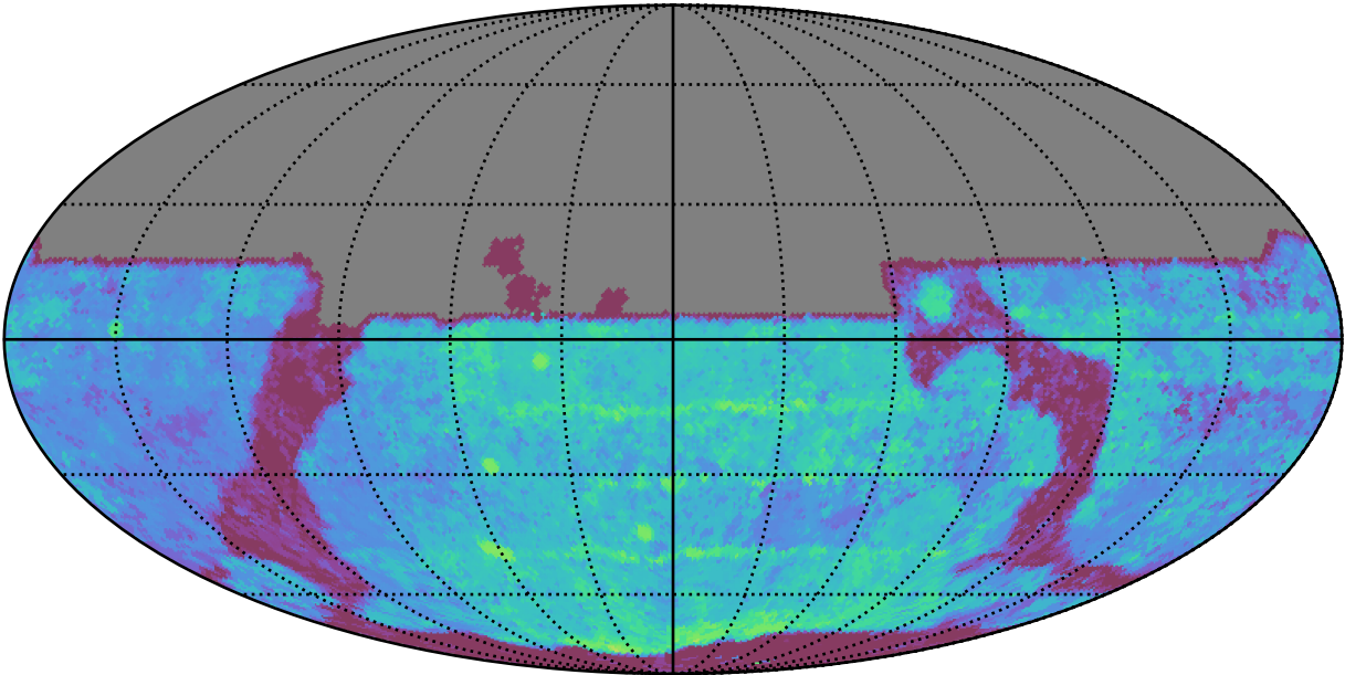
too_elab_heavy_r32_d3_ugrizy_v3.4_10yrs All sky y band: Median Season Length
